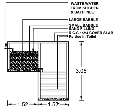
RECYCLING OF WASTE WATER FROM BATHROOM & KITCHEN
