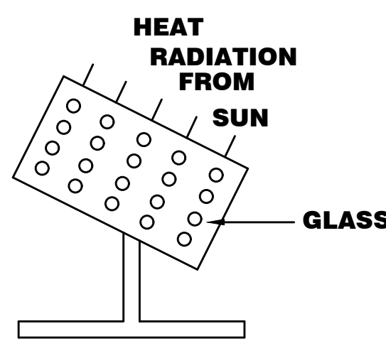
SOLAR SYSTEM
