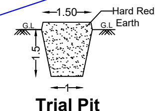
Trial Pit
