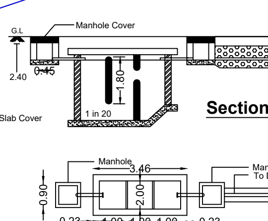
Details Of Septic TANK
