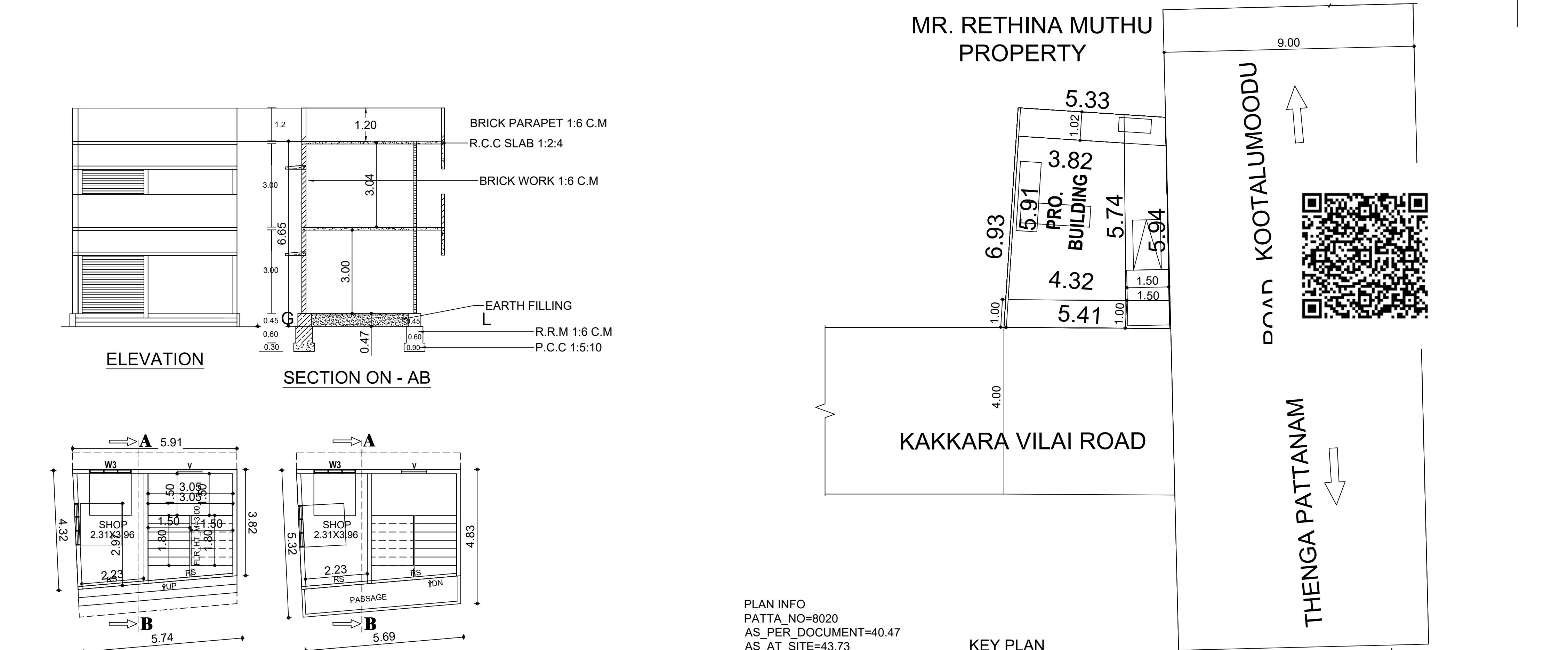
KEY PLAN SCALE 1:100 ALL DIMENSIONS ARE IN METRE
