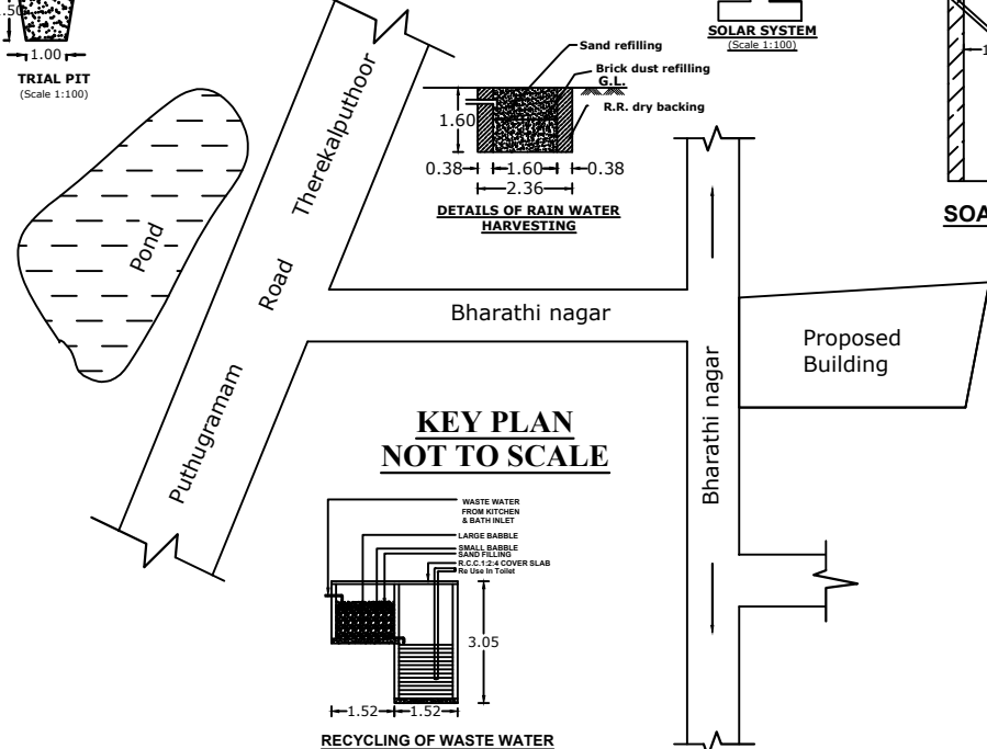
RECYCLING OF WASTE WATER FROM KITCHEN & BATHROOM
