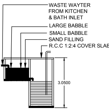
RECYCLING OF WASTE WATER TANK
