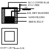
RAIN WATER HARVEST ARRANGEMENTS
