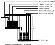
RECYCLING OF WASTE WATER FROM BATH
