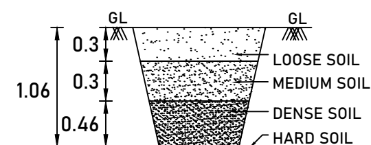
TRIAL-PIT
