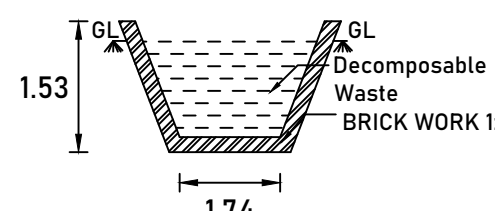
WASTE PIT
