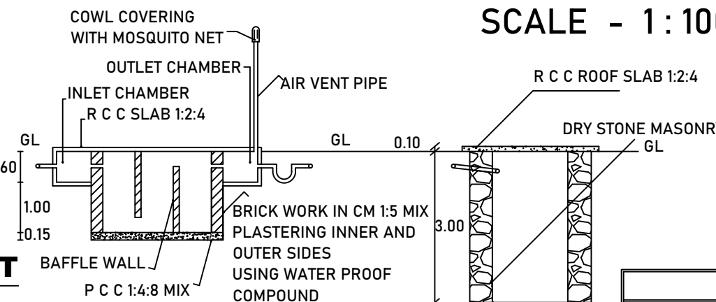
SECTION ON M-N
