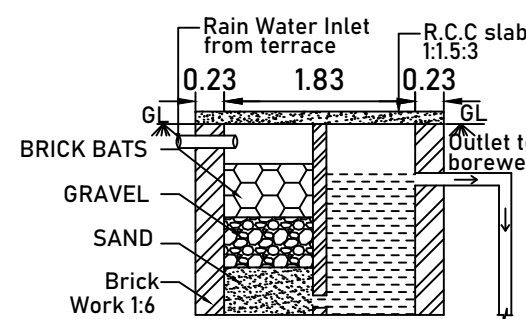
RAIN WATER HARVESTING - PIT
