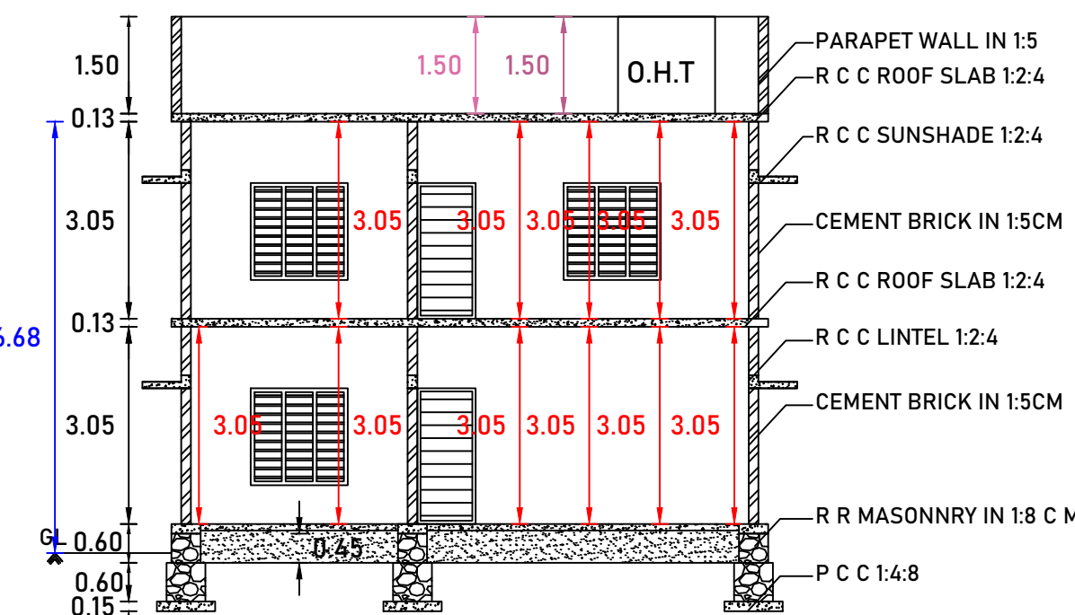
SECTION X-Y
