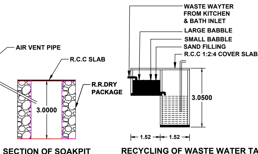
RECYCLING OF WASTE WATER TANK
