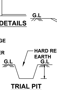
TRIAL PIT
