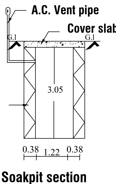
Soakpit section
