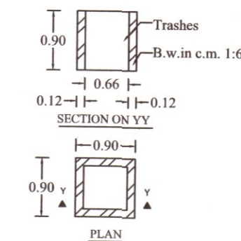
WASTE TRASH PIT
