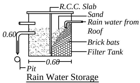
Rain Water Storage
