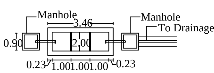
Details Of Septic Tank
