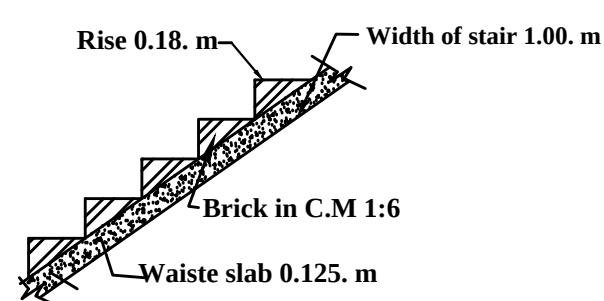
Stair Details
