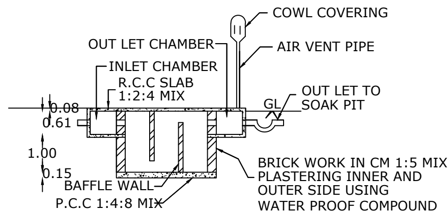
SECTION ON CD
