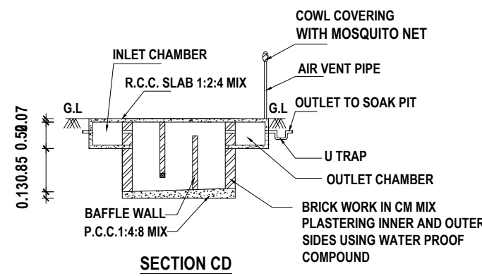
SECTION CD
