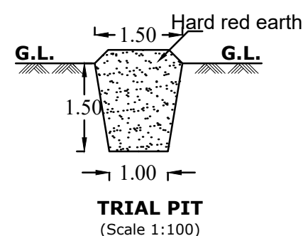
TRIAL PIT (Scale 1:100)
