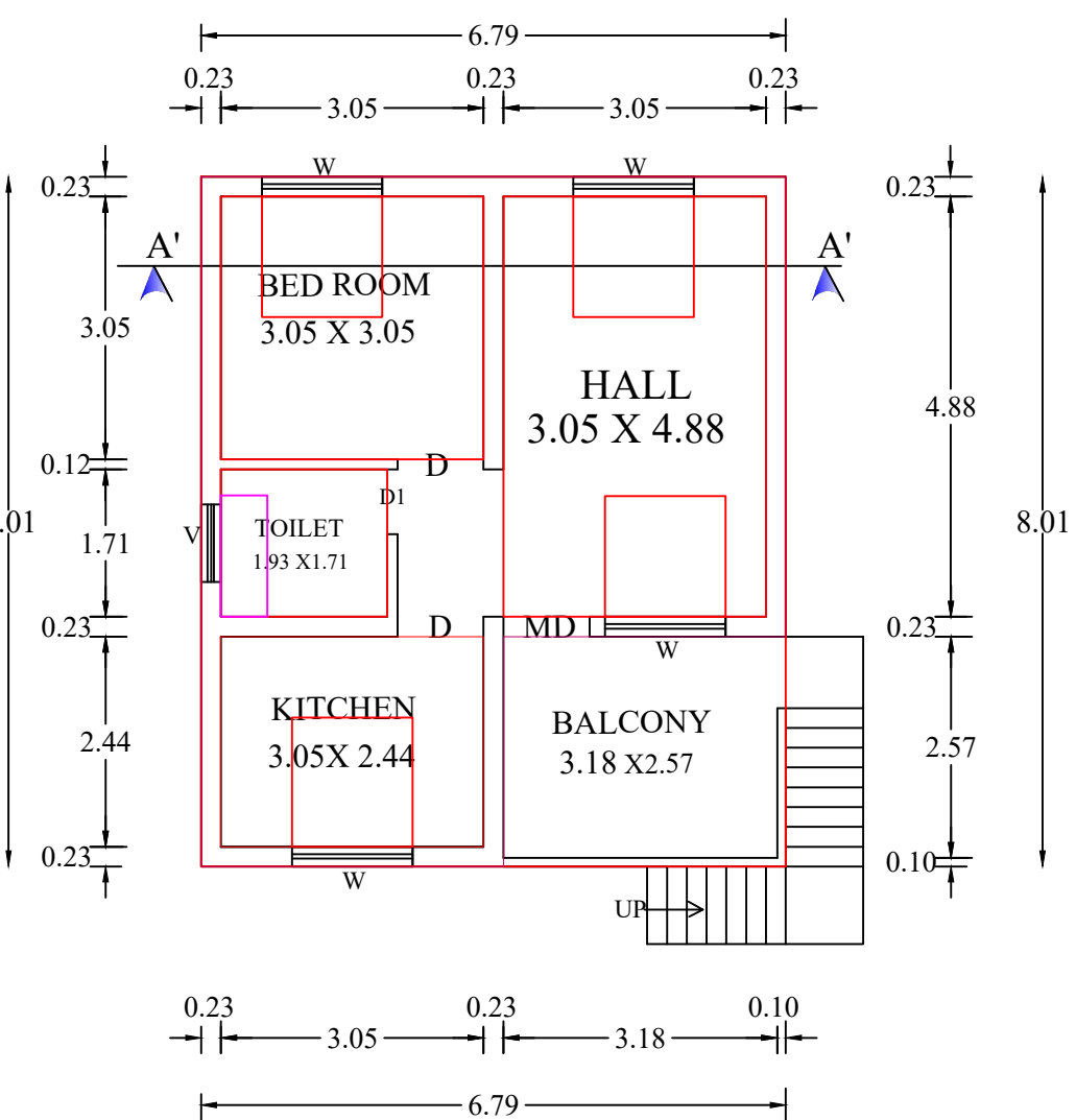
FIRST FLOOR
