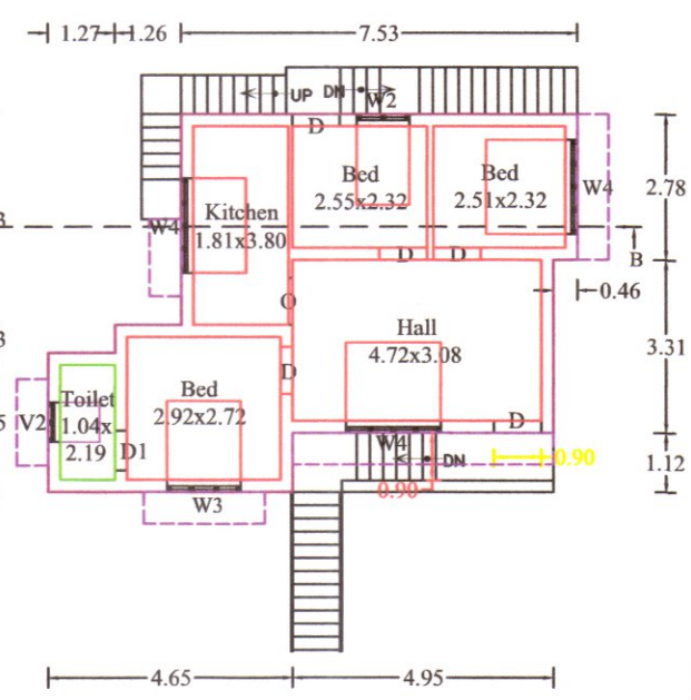
EXTENSION FIRST FLOOR PLAN
