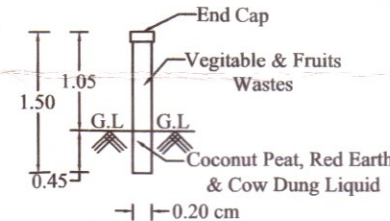
PIPE COMPOSTER
