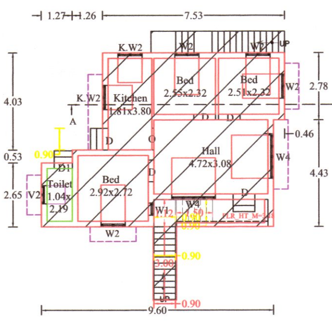
EXISTING GROUND FLOOR PLAN DOOR NO :- 12-99
