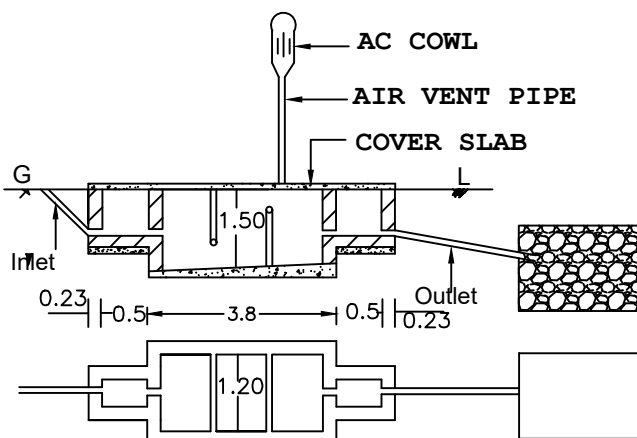
DETAILS OF SEPTIC TANK
