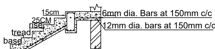
SECTION OF STAIRCASE
