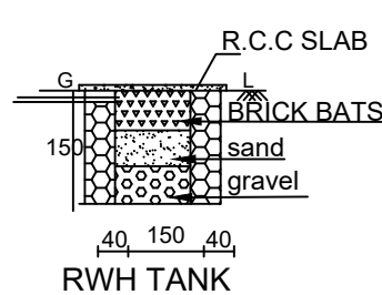
RWH TANK
