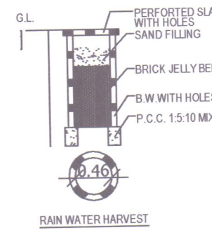
RAIN WATER HARVEST
