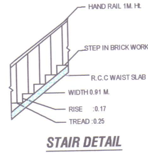
STAIR DETAIL
