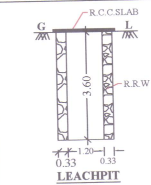
LEACH PIT
