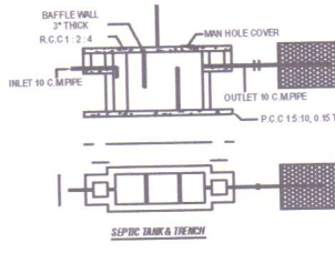
LEACH PIT
