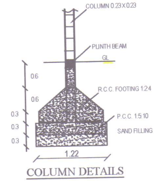
COLUMN DETAILS
