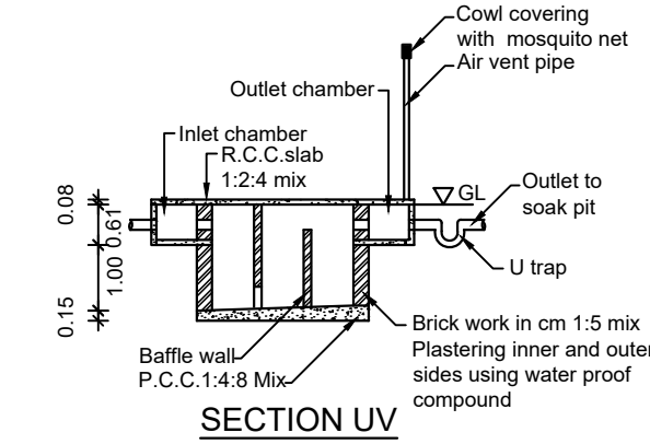
SECTION UV
