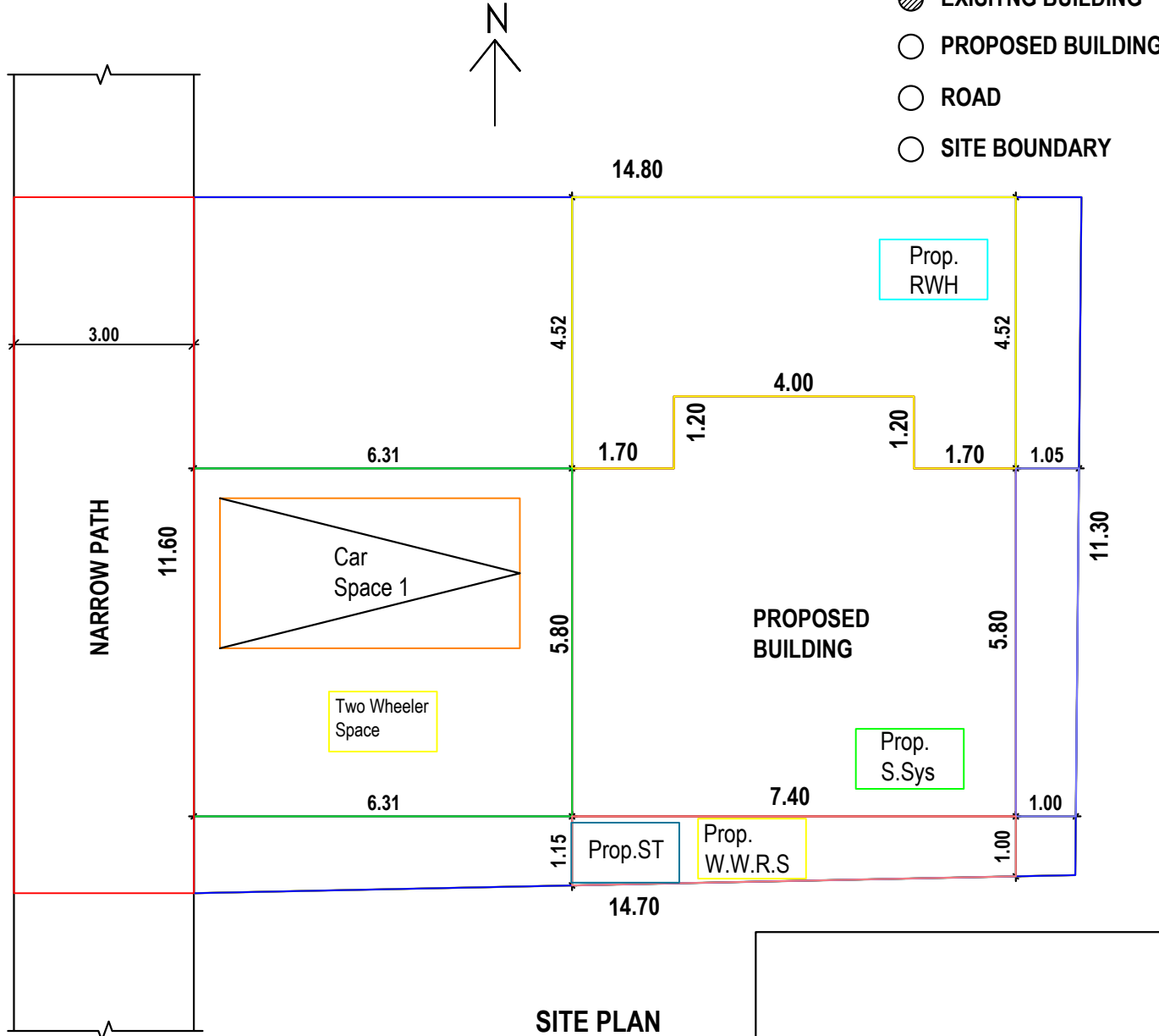
SITE PLAN
