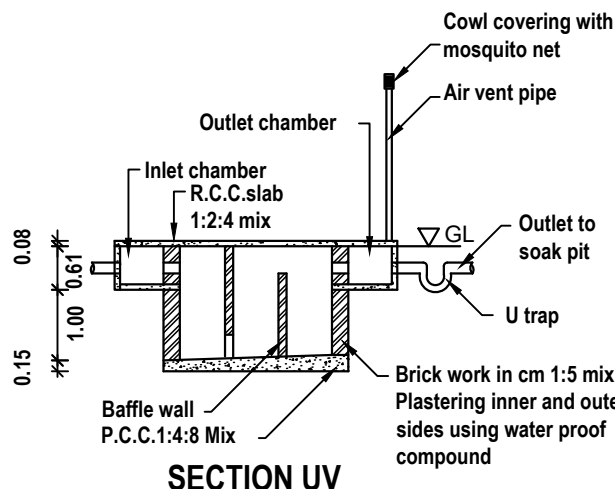
SECTION UV
