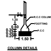
COLUMN DETAILS
