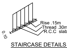
STAIRCASE DETAILS
