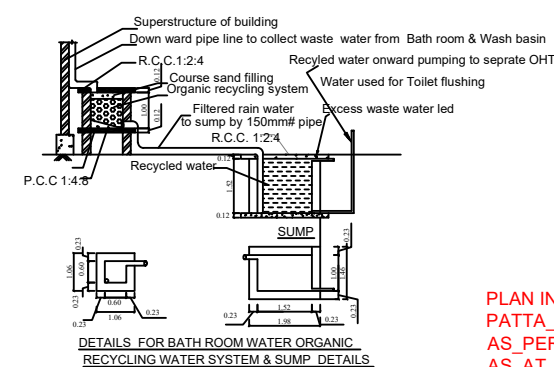
DETAILS FOR BATH ROOM ORGANIC RECYCLING WATER SYSTEM & SUMP DETAILS
