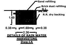
DETAILS OF SAND REFILLING SYSTEM
