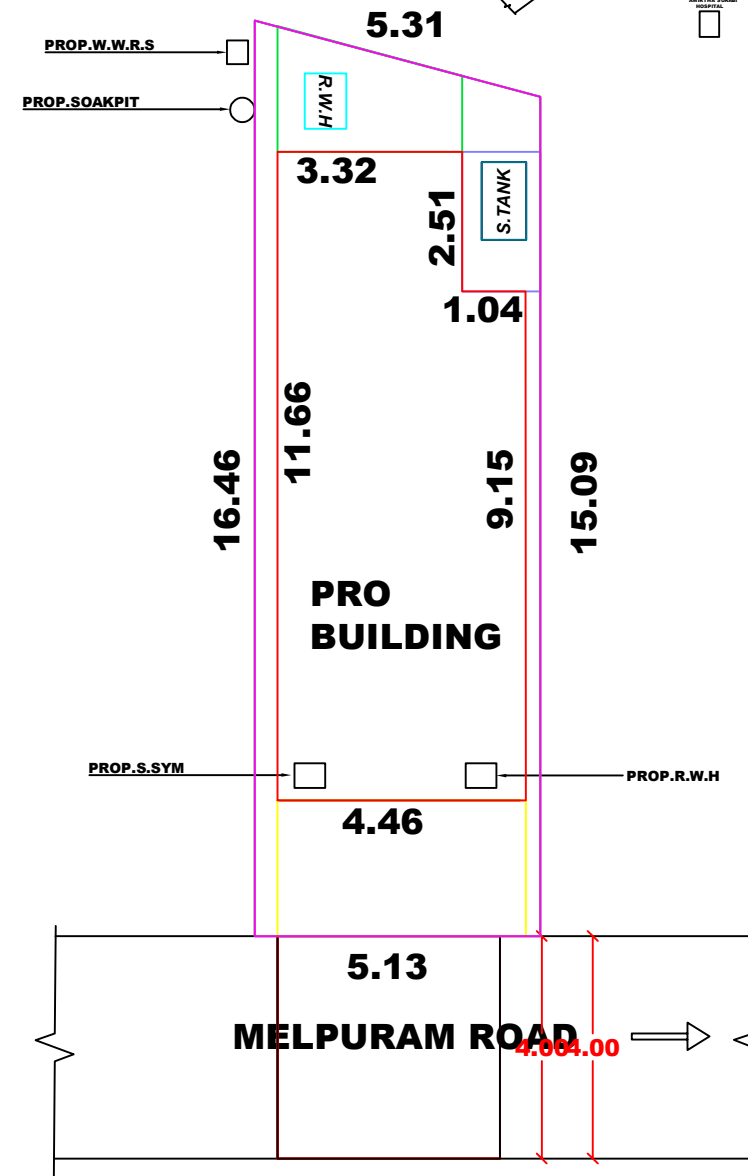
SITE PLAN
