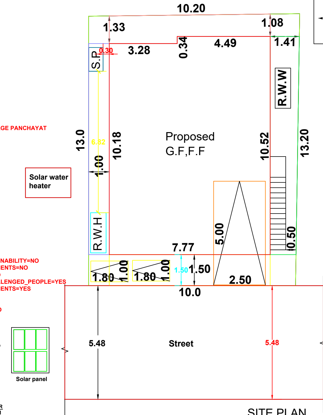
SITE PLAN
