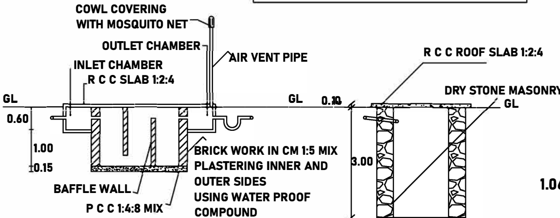
SECTION ON M-N
