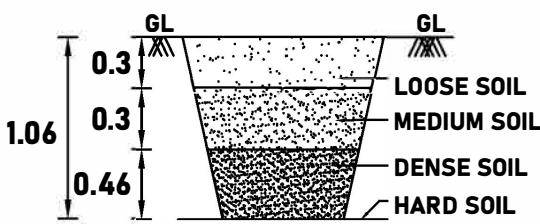
TRIAL-PIT
