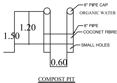
COMPOST PIT
