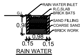
RAIN WATER
