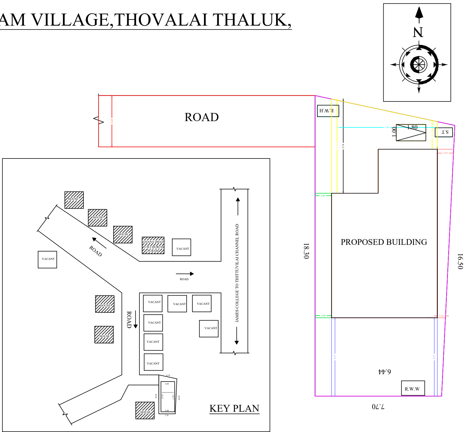
SITE PLAN
