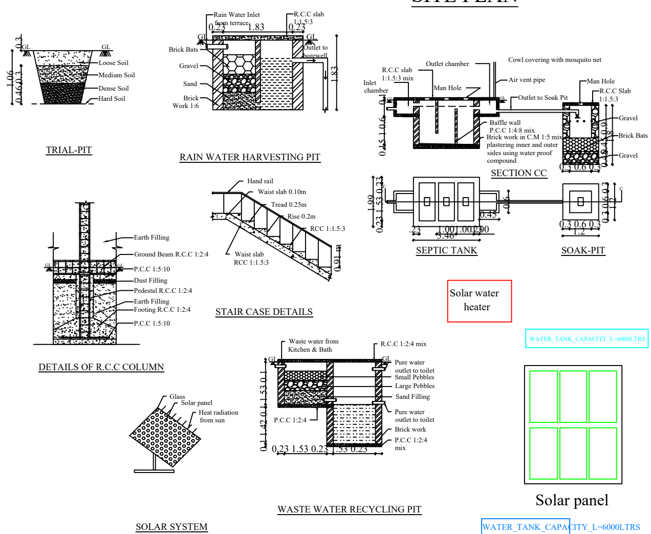
SITE PLAN
