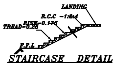
STAIRCASE DETAIL
