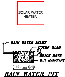
RAIN WATER PIT
