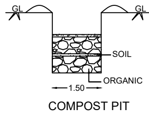
COMPOST PIT
