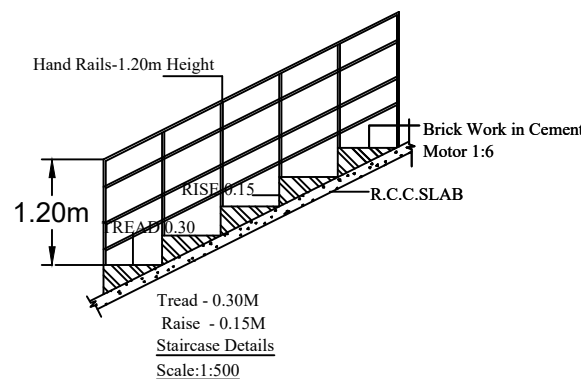
Staircase Details Scale:1:500
