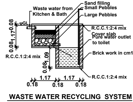
WASTE WATER RECYCLING SYSTEM
