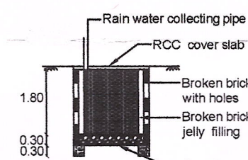
RAIN WATER HARVEST WELL SECTION
