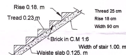
STAIR DETAILS
