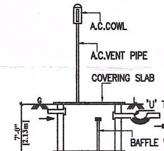
SEPTIC TANK C/S
