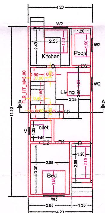
GROUND FLOOR PLAN [1:100]
