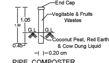
PIPE COMPOSTER
