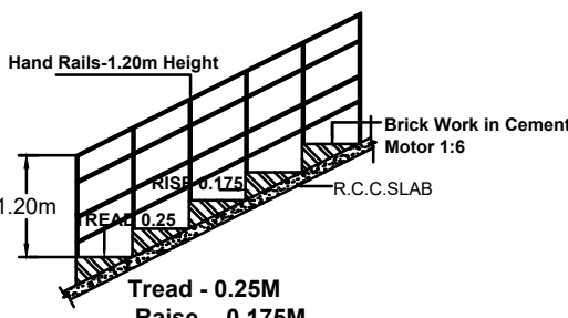
Tread - 0.25M Raise - 0.175M Staircase Details Scale:1:500
