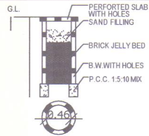
RAIN WATER HARVEST
