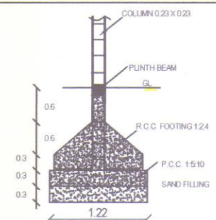
COLUMN DETAILS
