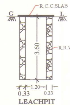
LEACHPIT
