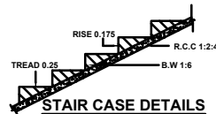
STAIR CASE DETAILS
