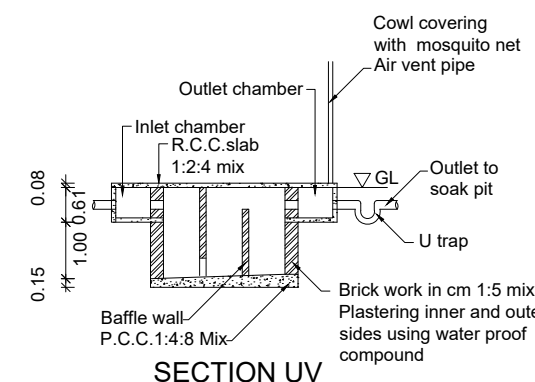
SECTION UV
