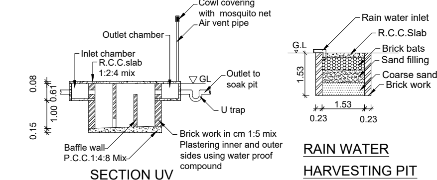
SECTION UV
