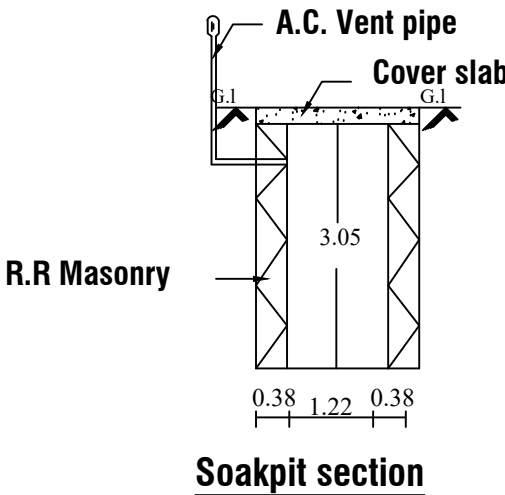
Soakpit section
