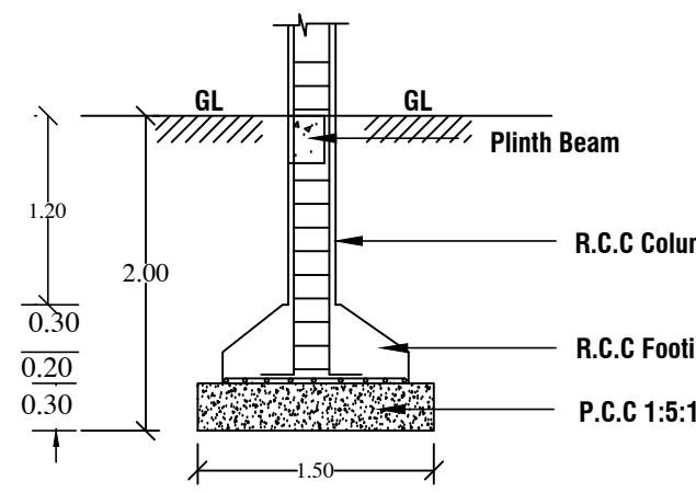
SECTION OF COLUMN
