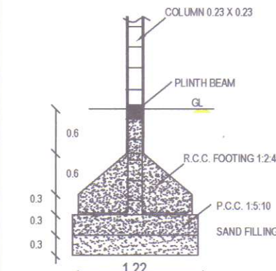
COLUMN DETAILS
