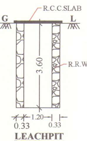
LEACHPIT
