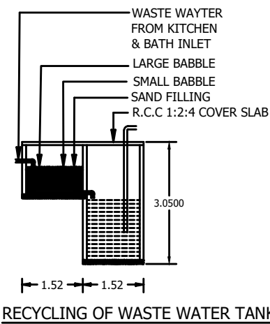
RECYCLING OF WASTE WATER TANK
