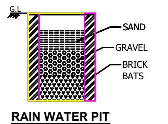
RAIN WATER PIT
