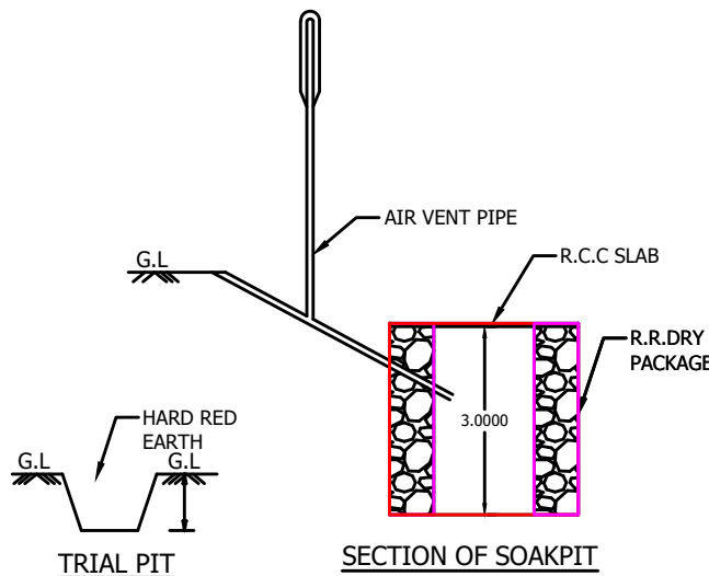
SECTION OF SOAKPIT
