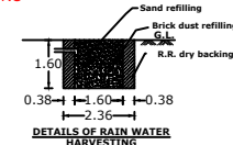
DETAILS OF RAIN WATER HARVESTING
