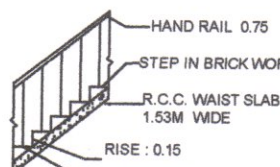
STAIR CASE SECTION
