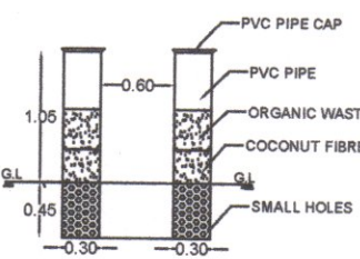
PIPE COMPOSIT PIT
