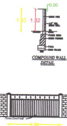
COMPOUND WALL DETAIL
