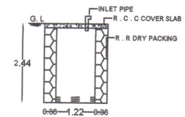
RAIN WATER STORAGE TANK SECTION
