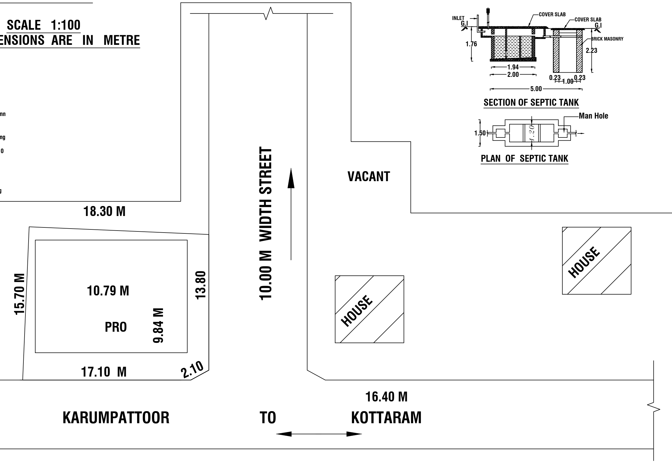
KEY PLAN
