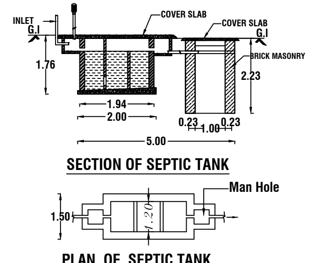
PLAN OF SEPTIC TANK
