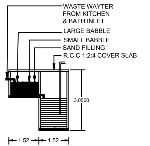
RECYCLING OF WASTE WATER TANK
