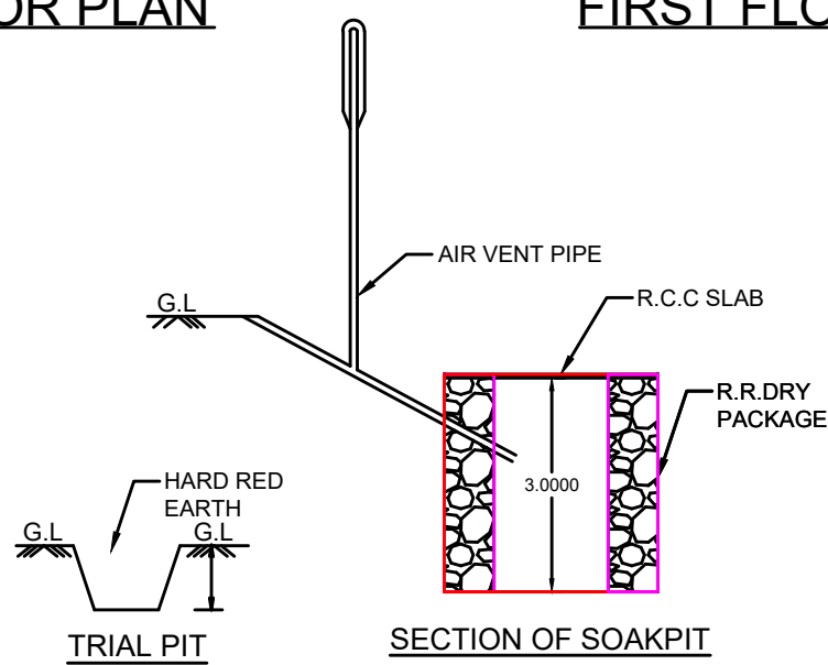
SECTION OF SOAKPIT
