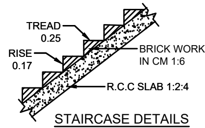
STAIRCASE DETAILS
