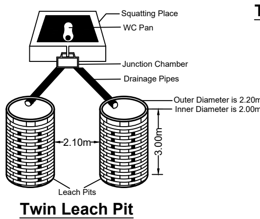
Twin Leach Pit
