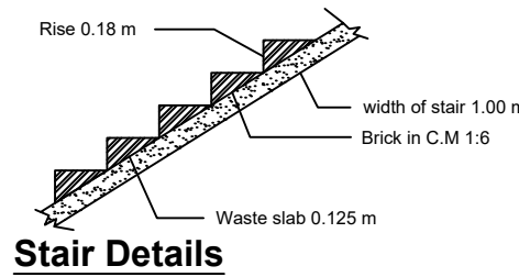
Stair Details
