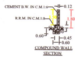
COMPOUND WALL SECTION
