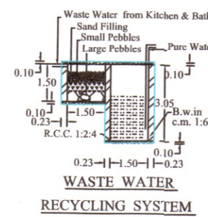
WASTE WATER RECYCLING SYSTEM
