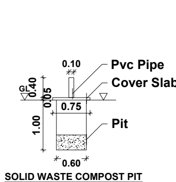
SOLID WASTE COMPOST PIT
