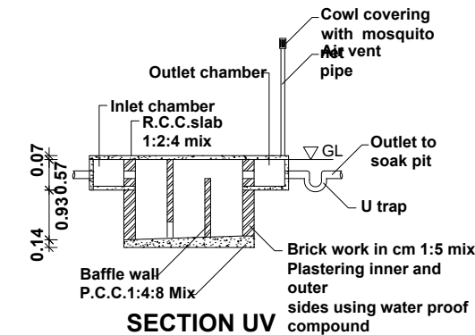
SECTION UV
