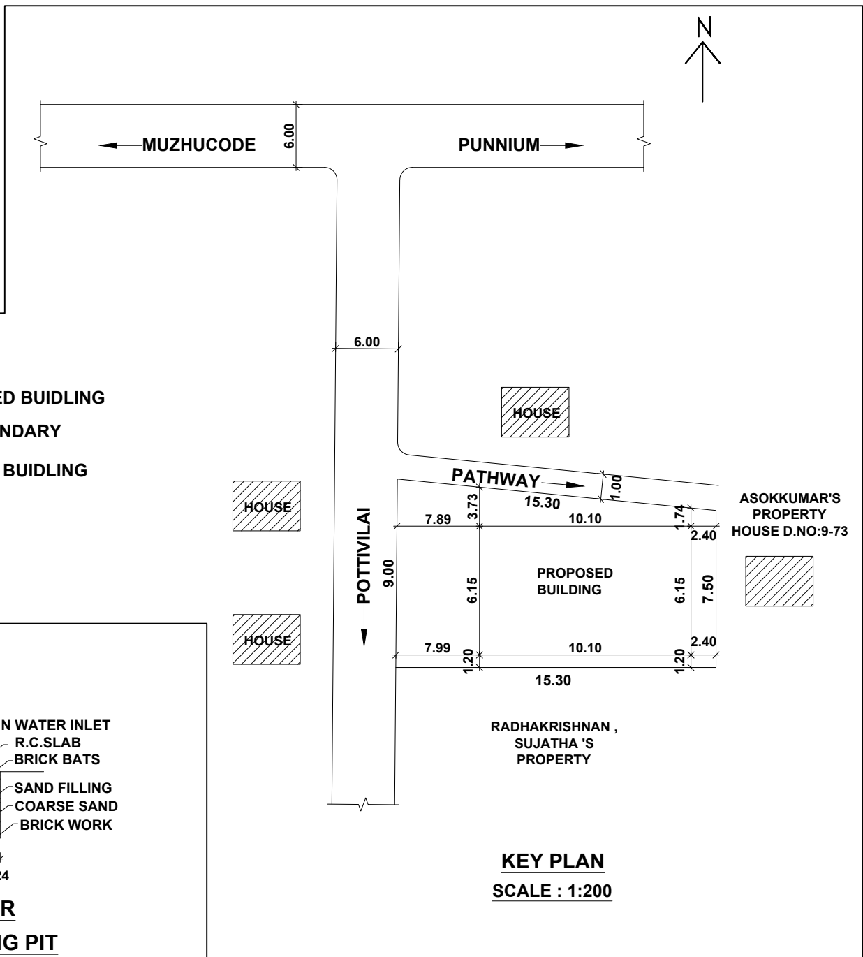
SITE PLAN
