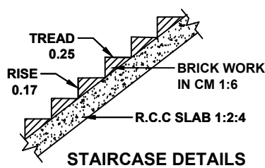
STAIRCASE DETAILS
