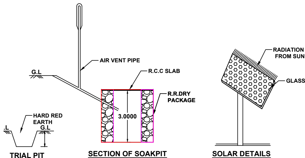
TRIAL PIT
